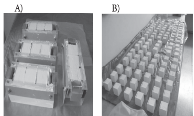
Figure 1. (A) Molding and (B) specimens for compressive strength and water absorption tests.
